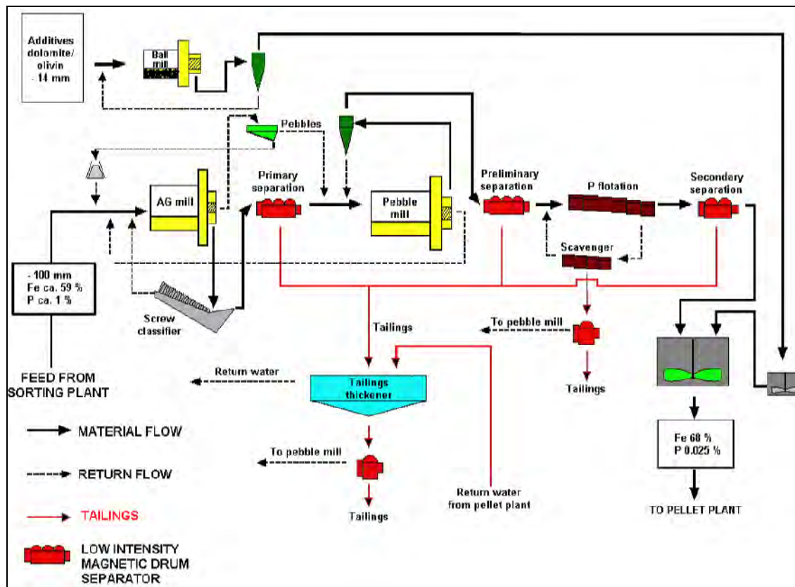
Figure 3.31: Kiruna concentrator
