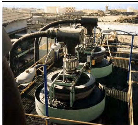
Figure 2.15: Mechanical flotation cell
