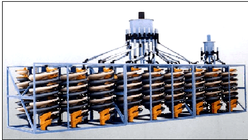
Figure 2.12: Spiral bank
